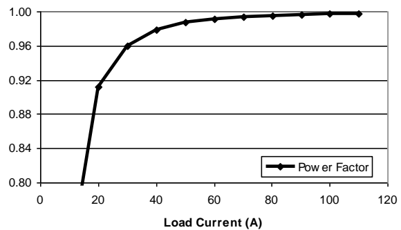
Power Factor vs Load at 54V
