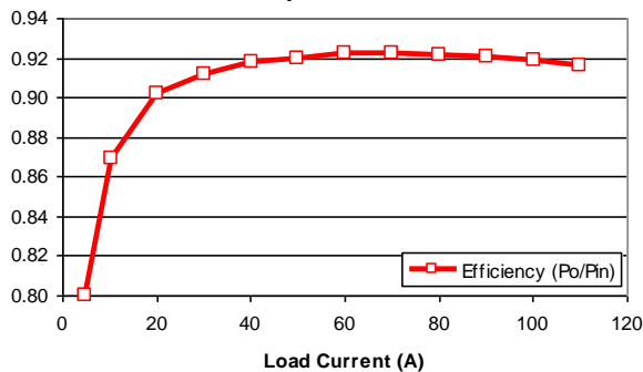
Efficiency vs Load at 54V
